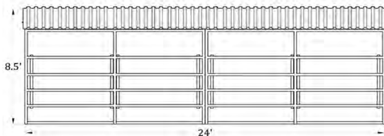
Side View (12'x12', 4 Stall Breezeway Barn)
