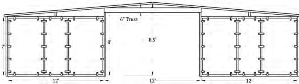
Front Elevation (12'x12', 8 Stall Plywood Ready Barn)
