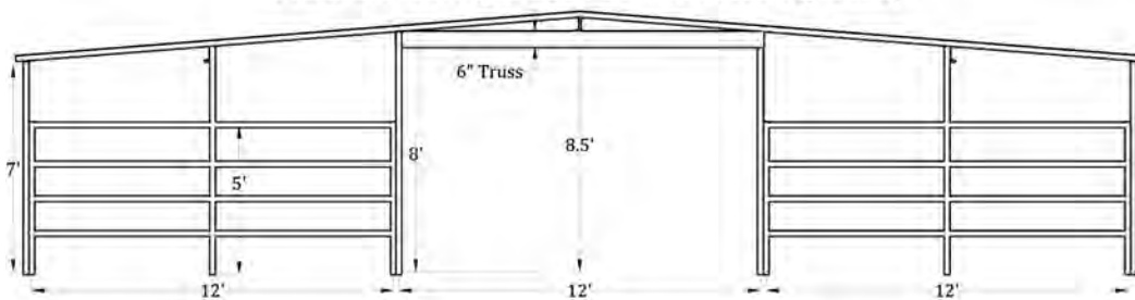
Front Elevation (12'x12', 6 Stall Breezeway Barn)
