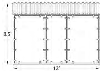
Side View (12'x12', 2 Stall Plywood Ready Barn)
