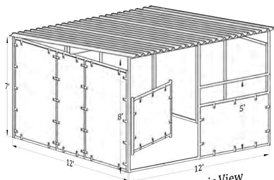
Isometric View (12'x12', Single Stall, Plywood Ready Shed) Total Area Covered = 12'x12'
