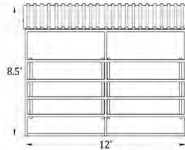
Side View (12'x12', 2 Stall Breezeway Barn)
