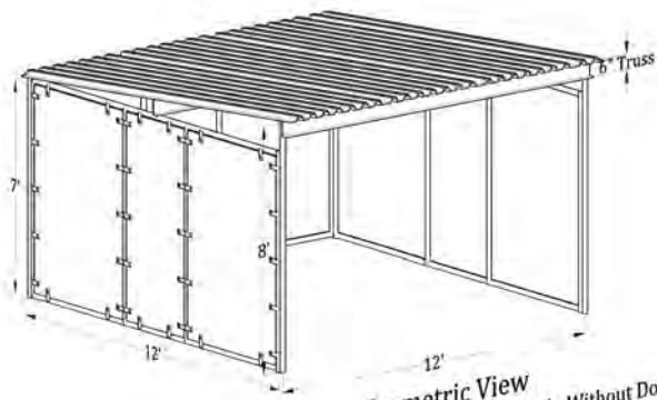
Isometric View (12'x12', Single Stall, Plywood Ready Shed - Without Door) Total Area Covered = 12'x12'
