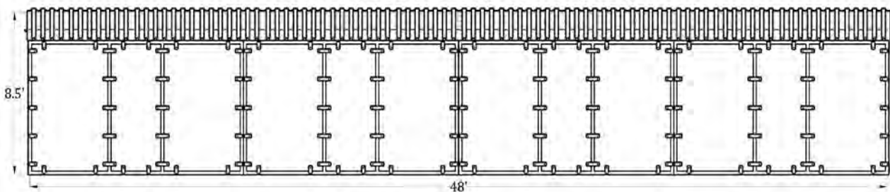
Side View (12'x12', 8 Stall Plywood Ready Barn)
