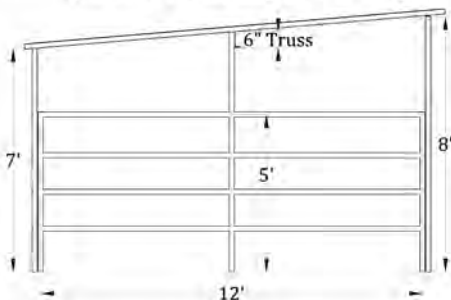
Side View (12'x12', 4-Rail, Single Stall Shed)
