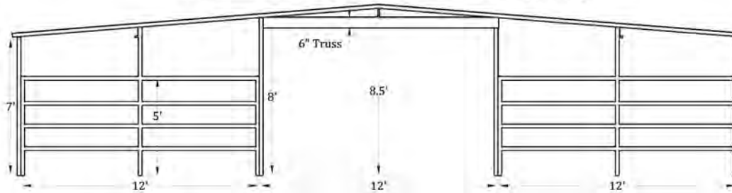
Front Elevation (12'x12', 4 Stall Breezeway Barn)
