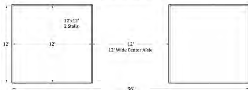
Top View (12'x12', 2 Stall Breezeway Barn) Total Area Covered = 12'x36'
