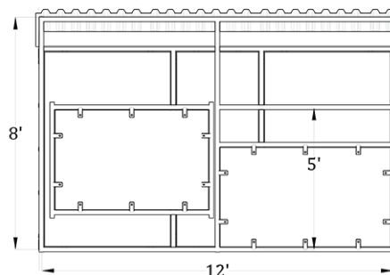
Front Elevation (12'x12', Single Stall, Plywood Ready Shed)
