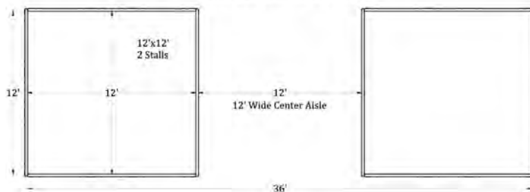
Top View (12'x12', 2 Stall Plywood Ready Barn) Total Area Covered = 12'x36'
