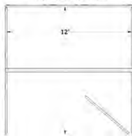
Top View (12'x12', Single Stall, Plywood Ready Shed) Total Covered Area = 12'x12'
