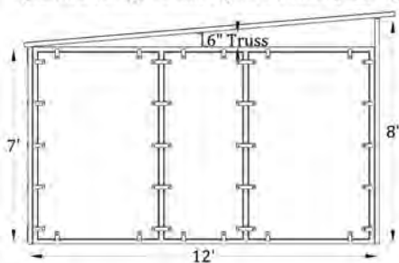
Side View (12'x12', Single Stall, Plywood Ready Shed)
