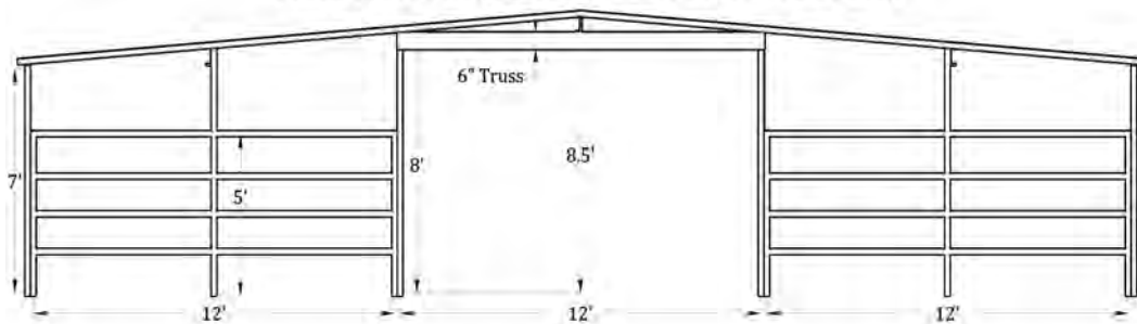
Front Elevation (12'x12', 8 Stall Breezeway Barn)
