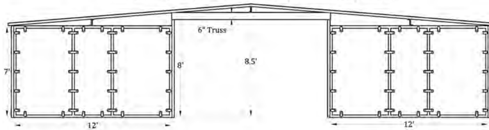
Front Elevation (12'x12', 2 Stall Plywood Ready Barn)
