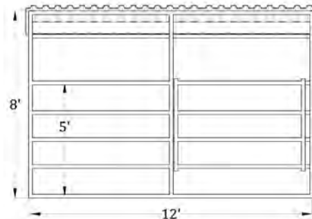
Front Elevation (12'x12', 4-Rail, Single Stall Shed)
