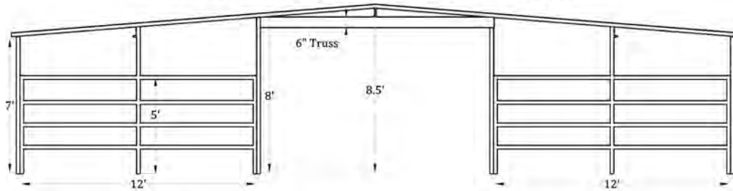
Front Elevation (12'x12', 2 Stall Breezeway Barn)
