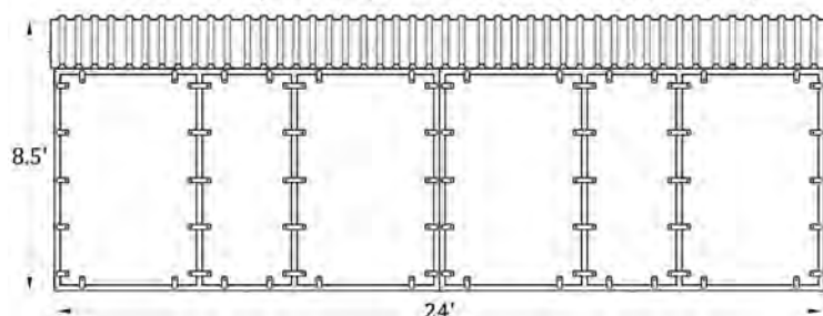
Side View (12'x12', 4 Stall Plywood Ready Barn)
