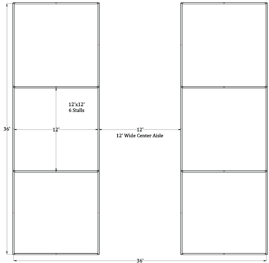
Top View (12'x12', 6 Stall Breezeway Barn) Total Area Covered = 36'x36'
