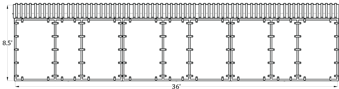
Side View (12'x12', 6 Stall Plywood Ready Barn)
