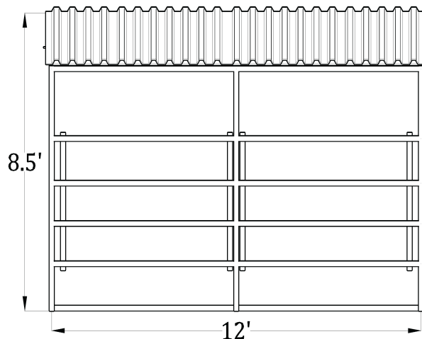
Side View (12'x12', 2 Stall Breezeway Barn)
