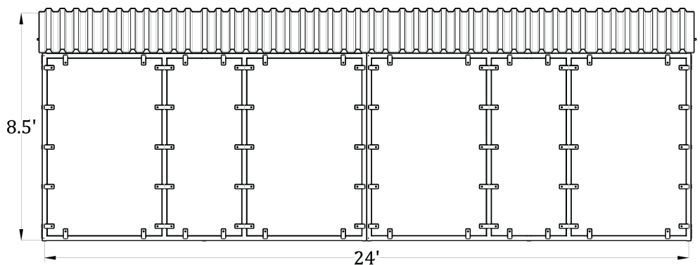
Side View (12'x12', 4 Stall Plywood Ready Barn)
