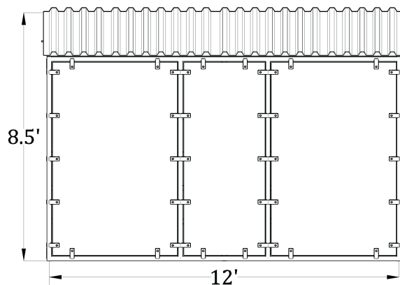
Side View (12'x12', 2 Stall Plywood Ready Barn)
