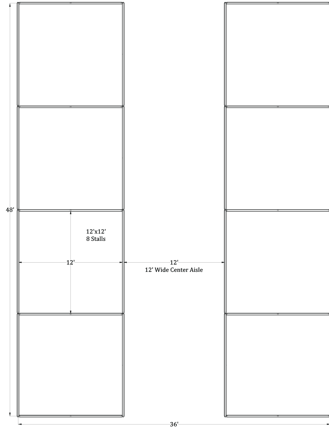
Top View (12'x12', 8 Stall Breezeway Barn) Total Area Covered = 48'x36'
