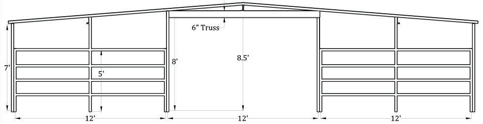
Front Elevation (12'x12', 6 Stall Breezeway Barn)
