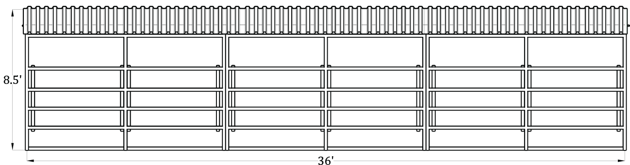
Side View (12'x12', 6 Stall Breezeway Barn)
