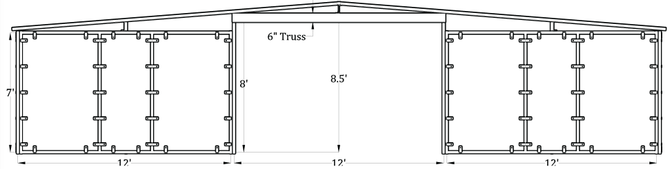
Front Elevation (12'x12', 6 Stall Plywood Ready Barn)
