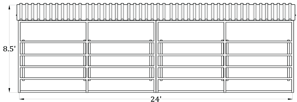
Side View (12'x12', 4 Stall Breezeway Barn)
