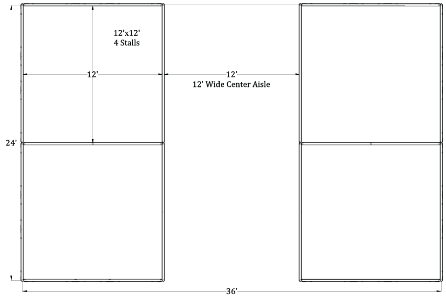
Top View (12'x12', 4 Stall Plywood Ready Barn) Total Area Covered = 24'x36'
