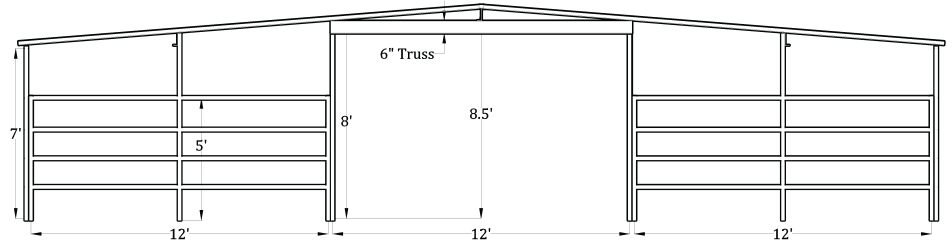
Front Elevation (12'x12', 8 Stall Breezeway Barn)
