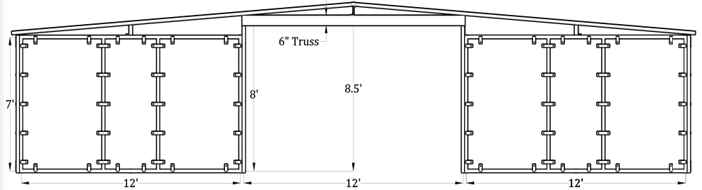
Front Elevation (12'x12', 8 Stall Plywood Ready Barn)
