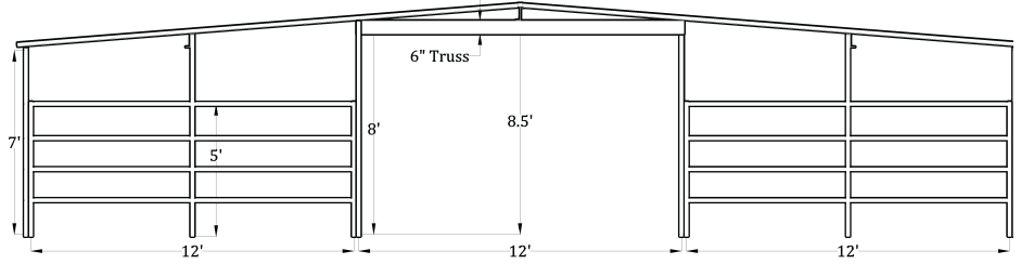
Front Elevation (12'x12', 4 Stall Breezeway Barn)
