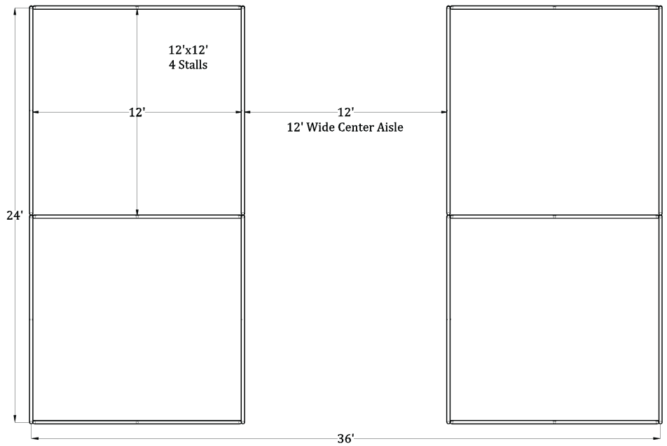
Top View (12'x12', 4 Stall Breezeway Barn) Total Area Covered = 24'x36'
