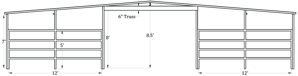
Front Elevation (12'x12', 2 Stall Breezeway Barn)
