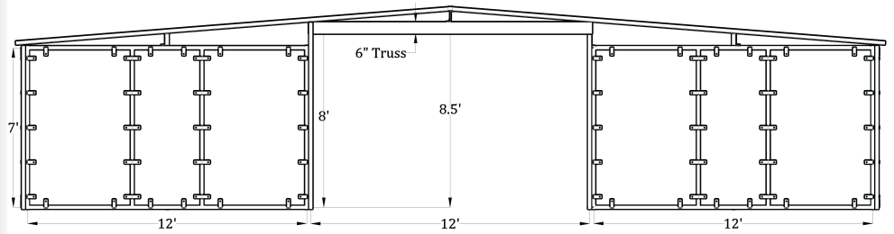
Front Elevation (12'x12', 4 Stall Plywood Ready Barn)
