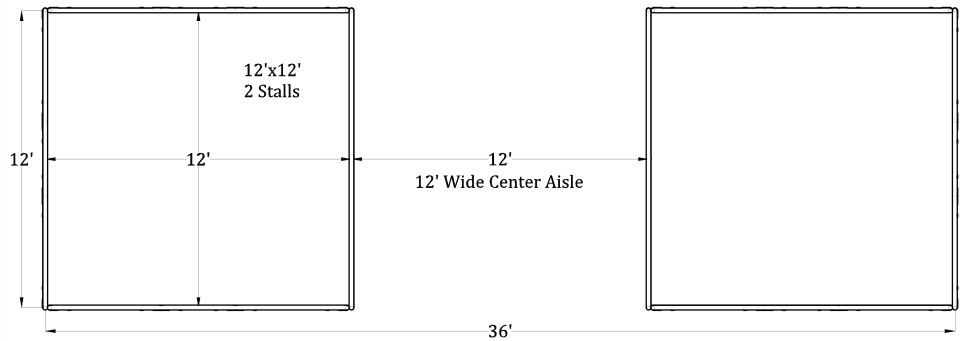
Top View (12'x12', 2 Stall Plywood Ready Barn)
