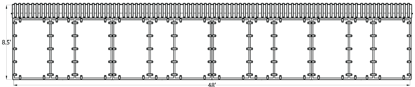
Side View (12'x12', 8 Stall Plywood Ready Barn)
