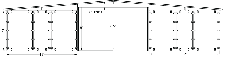
Front Elevation (12'x12', 2 Stall Plywood Ready Barn)
