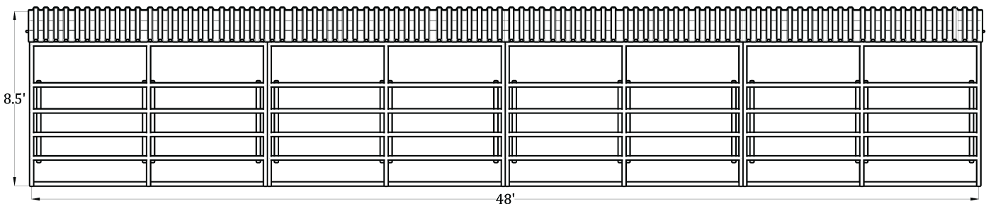
Side View (12'x12', 8 Stall Breezeway Barn)
